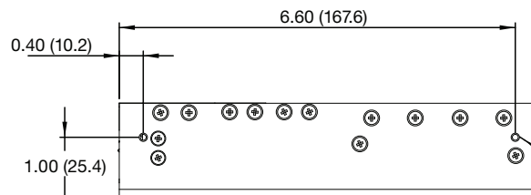
3 Way DINKLE DT-2C-B14W-03 M3 SCREWS IN 3 POSITIONS TORQUE TO 7lbs-in (80 cNm) MAX.
